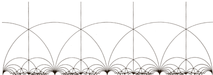
Figure 3.14. Tesselation of H for SL(2, \mathbb{Z}) . (Computer drawing by the UCSD VAX and Mark Eggert.)
