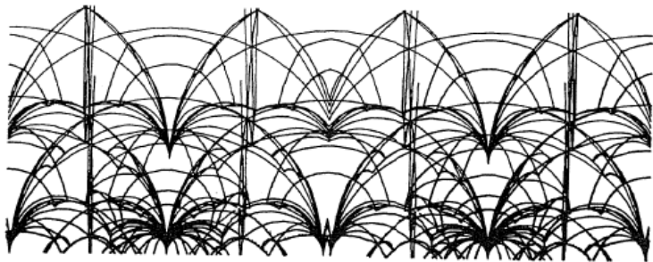
Figure 5.5. Tessellation of the quaternionic upper half plane from SL(2, \mathbb{Z}[i]) in stereo. (Drawn by the UCSD VAX computer and Mark Eggert.)
